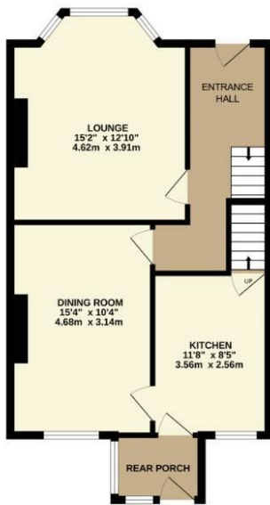
GROUND FLOOR 564 sq.ft. (52.4 sq.m.) approx.
